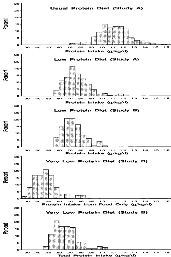
Figure 1. Distribution of protein intakes during follow-up in the MDRD Study. Panels show the distribution of mean protein intake during follow-up for patients assigned to the usual, low, and very low protein diet groups. Mean protein intake is defined as the average of all values for protein intake, estimated from the urine urea nitrogen beginning at the second follow-up visit. Protein intakes are factored by standard body weight. (A) Study A, usual protein diet (prescribed protein intake 1.3 g/kg per d, achieved group mean protein intake 1.11 g/kg per d). (B) Study A, low protein diet (prescribed protein intake 0.58 g/kg per d; achieved group mean protein intake 0.77 g/kg per d). (C) Study B, low protein diet (prescribed protein intake 0.58 g/kg per d, achieved group mean protein intake 0.73 g/kg per d). (D) Study B, very low protein diet supplemented with ketoacids and amino acids (prescribed protein intake from food 0.28 g/kg per d, achieved group mean protein intake from food 0.48 g/kg per d). To estimate protein intake from food, the nitrogen contained in the ketoacid–amino acid mixture was subtracted from the urinary urea nitrogen. (E) Study B, very low protein diet supplemented with ketoacids and amino acids (prescribed protein intake from food and supplements 0.56 g/kg per d, achieved group mean total protein intake from food and supplements 0.66 g/kg per d). Reprinted with permission from J Am Soc Nephrol (8) and Am J Kidney Dis (9).
