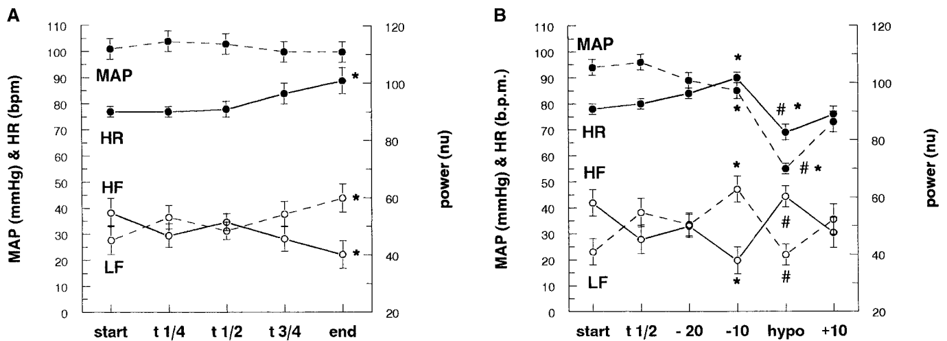
Figure 2. MAP, HR, and low frequency (LF) and high frequency (HF) power (nu, normalized units) in dialysis sessions without (A) and with (B) symptomatic hypotension. Start, start of dialysis; end, end of dialysis. Panel A: t 1 / 4 , t 1 / 2 , and t 3 / 4 : 25, 50, and 75% of dialysis duration, respectively. Panel B: t 1 / 2 , halfway between start of dialysis and moment of hypotension; -20, -10, 20 min and 10 min before hypotension, respectively; hypo, moment of hypotension. *P < 0.05 versus baseline; #P < 0.05 versus -10 min.
