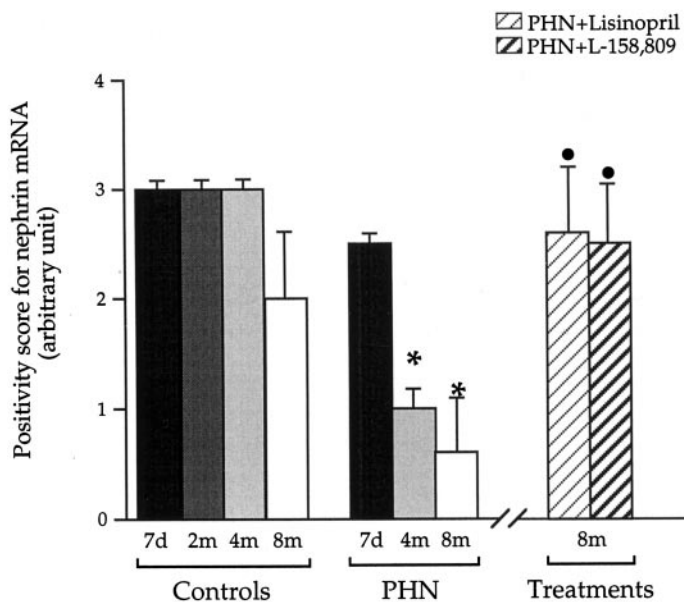
Figure 2. Intensity score (arbitrary units) of nephrin mRNA staining in control and PHN rats studied at different time points. The effect of lisinopril and L-158,809 chronically given to PHN rats on nephrin gene expression is also shown. *, P < 0.05 versus controls at respective time; ●, P < 0.05 versus PHN 8 mo.
