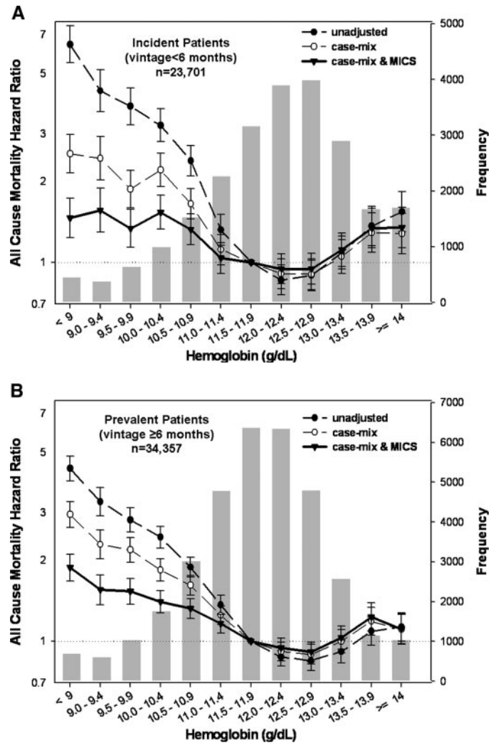
Figure 2. Comparing “incident” (vintage <6 mo, n = 23,701 ; top) and “prevalent” (vintage \geq 6 mo, n = 34,357 ; bottom) MHD patients with regard to the association between the time-varying blood hemoglobin values and the relative risk for all-cause death during a 2-yr interval (July 2001 to June 2003).
