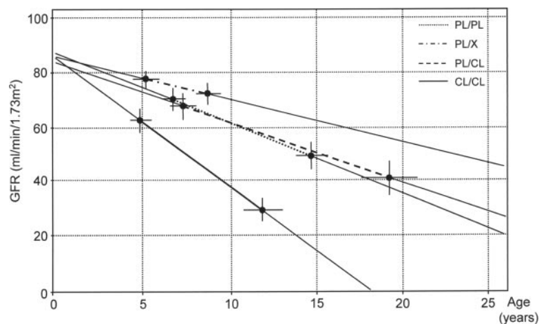
Figure 5. Progression of renal failure over time in FHHNC according to the mutation category. Data are means \pm SEM.
